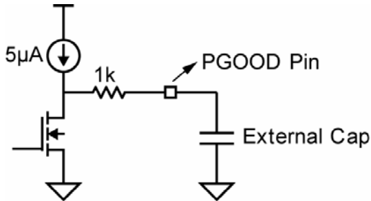
Figure 1. Power Good Circuit
